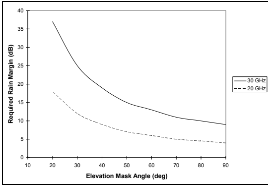
Figure 1. Required Rain Margin (Region D2, 99.9% Availability)
