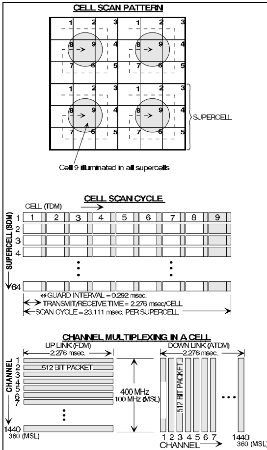
Figure 7. Standard & Mobile Terminal Multiple Access
