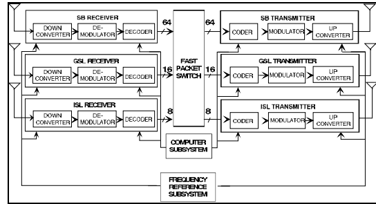
Figure 9. Communications Payload
